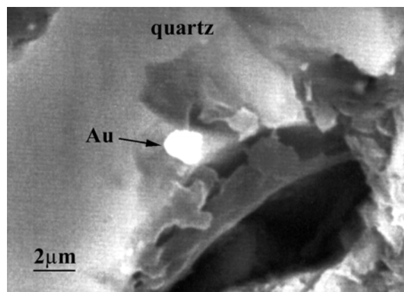
Fig.10. Native gold lamella on second-generation quartz. Grey, argillic silica. R4-79.4m. Au: 0.02 g/t. BSE image.
