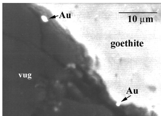
Fig.9. Native gold on goethite at a vug. Limonitic breccia, R4-45.4m. Au: 0.35 g/t. BSE image.
