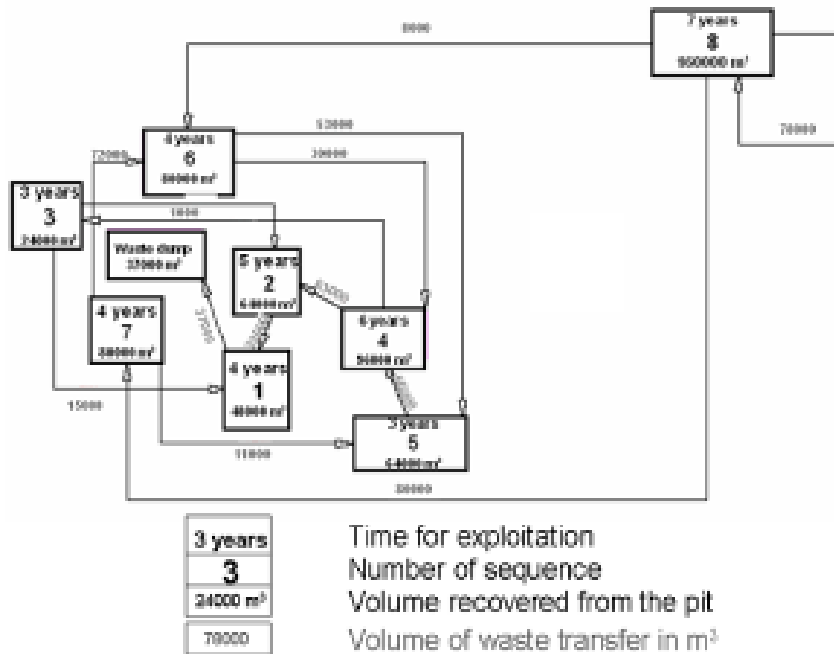
Fig. 13. Exploitation sequence.
