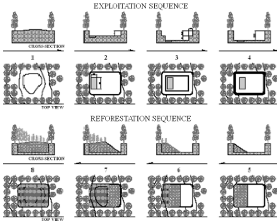
Fig. 14. Exploitation and reforestation sequence of a pit.
