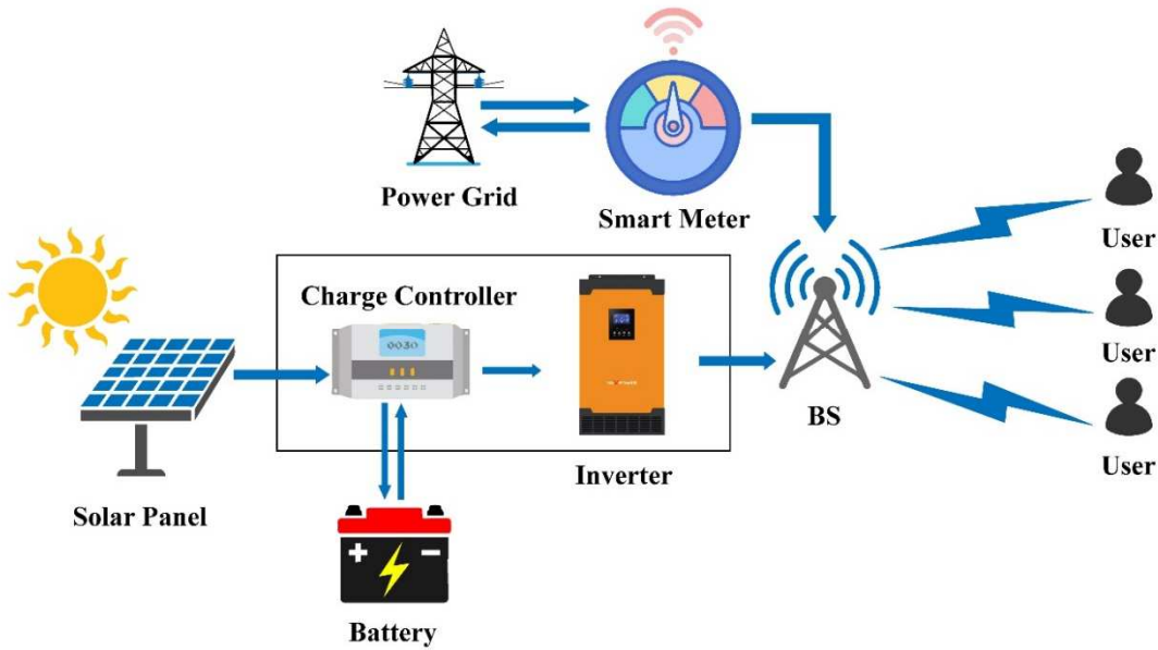
Fig. 2. A hybrid energy power base station.
