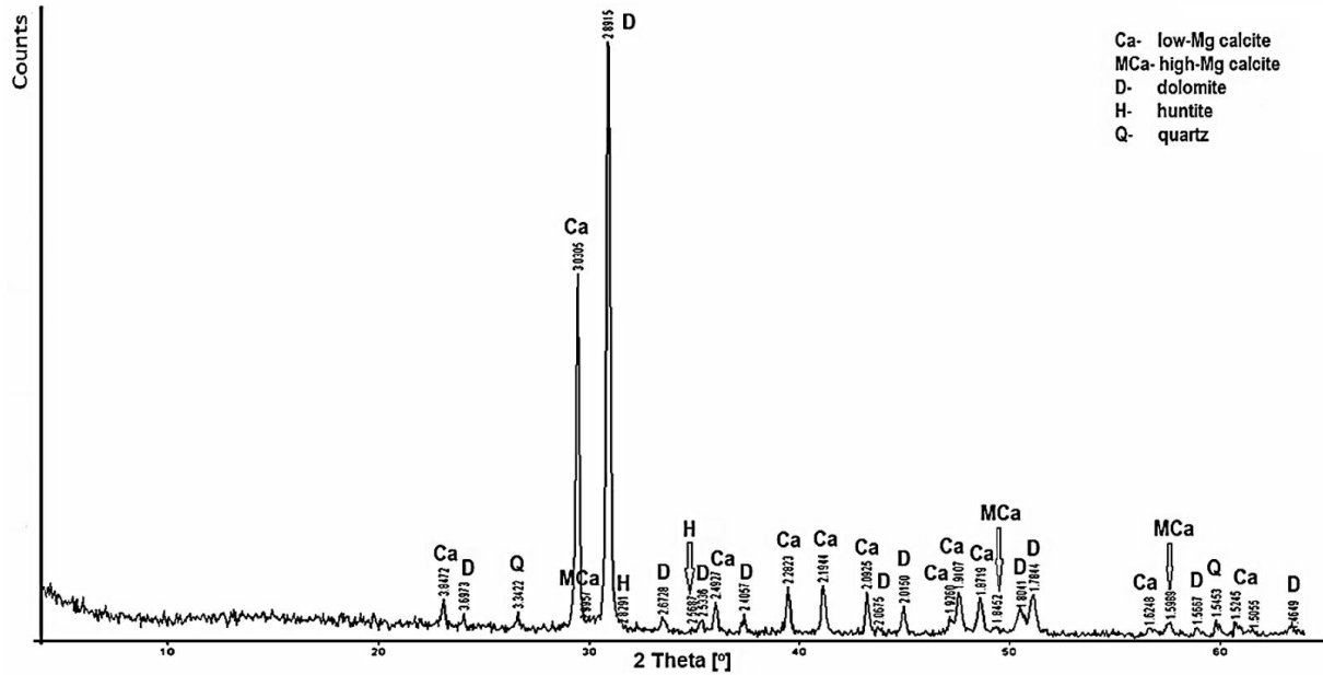
Fig. 8. X-ray diffraction pattern of sample SO14 (Karchowice Limestone) (Stanienda, 2013b, 2016a).
