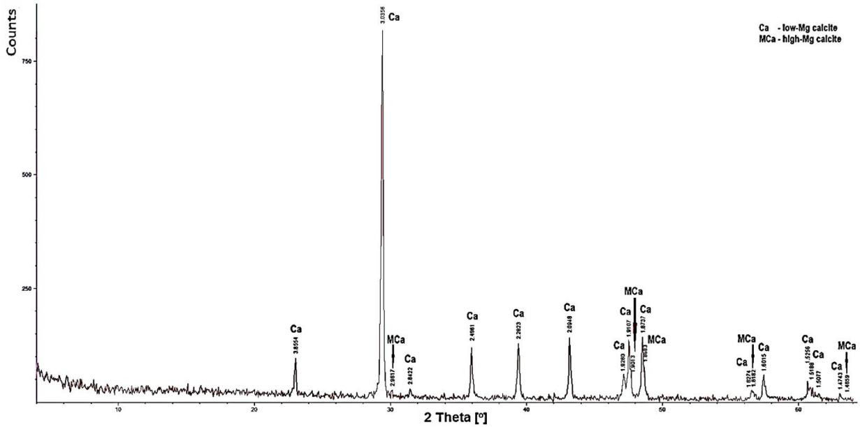
Fig. 5. X-ray diffraction pattern of sample W1 (Góraźdze Limestone).
