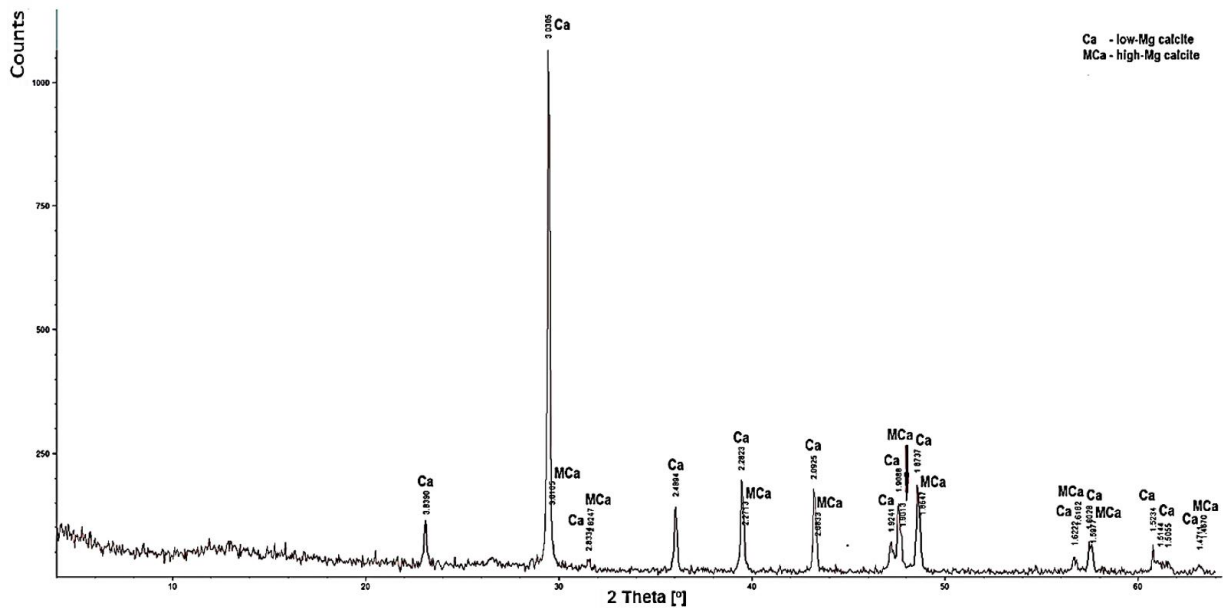
Fig. 4. X-ray diffraction pattern of sample SA5 (Górażdże Limestone).
