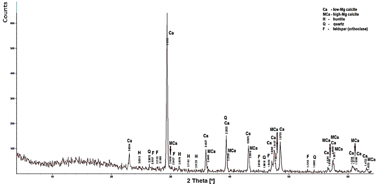
Fig. 7. X-ray diffraction pattern of sample S7 (Dziewkowiec Limestone).
